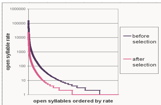
Figure 3. Distribution of open syllables in initial and output text corpora.
