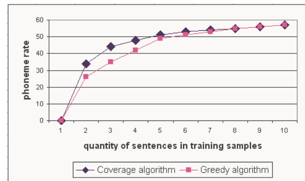
Figure 1. Dynamics of new phoneme appearance with processed sentences growing for greedy algorithm and coverage algorithm
